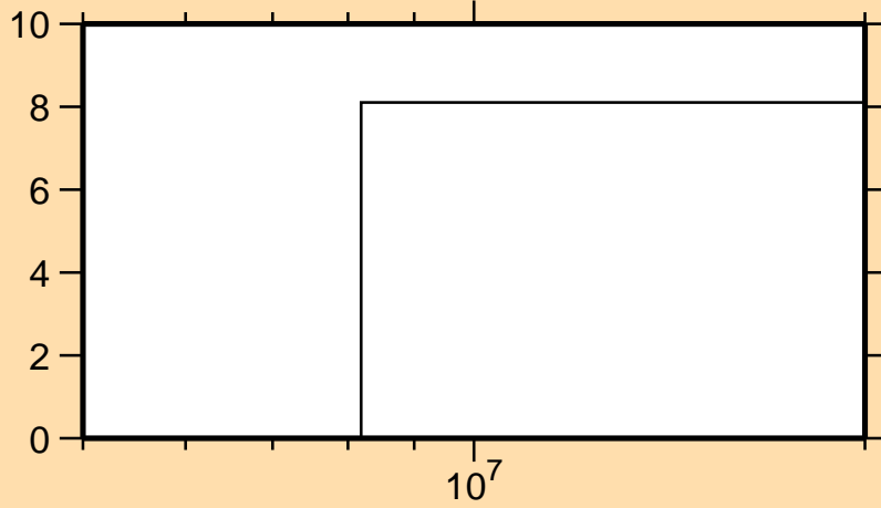
\Delta\sigma/\sigma vs. E for ^{48}\text{Ti}(n,2n)
