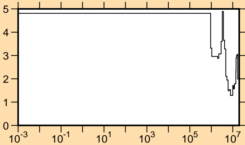
\Delta v/v vs. E for ^{240}\text{Pu} (prompt \nu )
