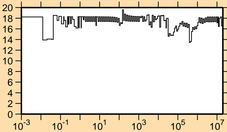
\Delta\sigma/\sigma vs. E for ^{59}\text{Co}(n,\gamma)
