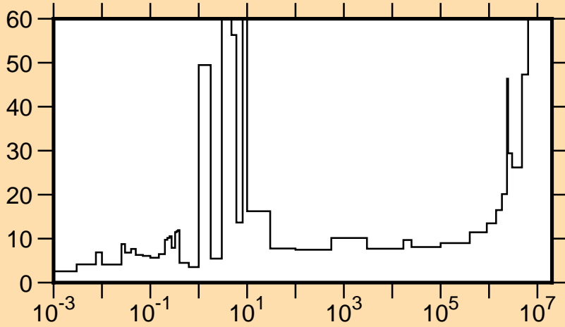
\Delta\sigma/\sigma vs. E for ^{185}\text{Re}(n,\gamma)
