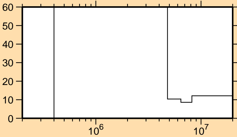
\Delta\sigma/\sigma vs. E for ^{62}\text{Ni}(n,\alpha)
