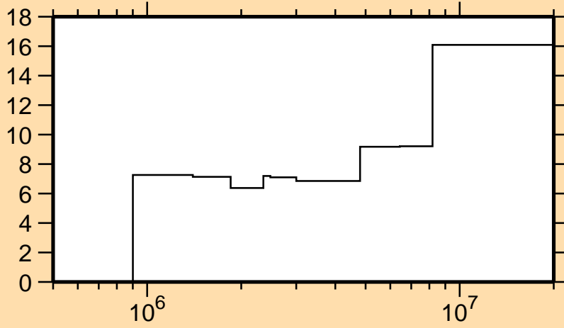
\Delta\sigma/\sigma vs. E for ^{62}\text{Ni}(n,\text{inel.})
