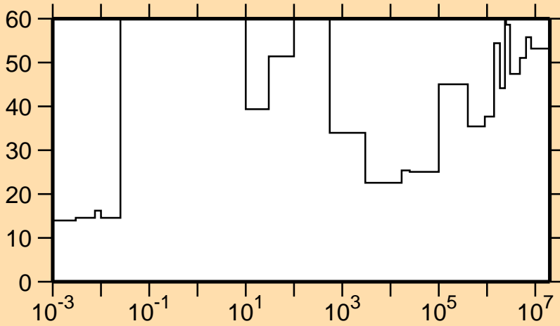
\Delta\sigma/\sigma vs. E for ^{62}\text{Ni}(n,\gamma)
