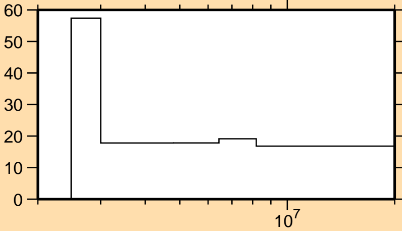
\Delta\sigma/\sigma vs. E for ^{62}\text{Ni}(n,n\text{cont.})
