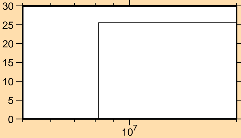
\Delta\sigma/\sigma vs. E for ^{62}\text{Ni}(n,d)
