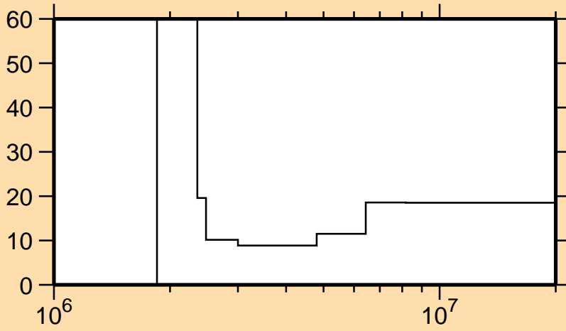
\Delta\sigma/\sigma vs. E for ^{62}\text{Ni}(n,n_3)
