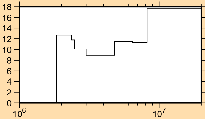
\Delta\sigma/\sigma vs. E for ^{62}\text{Ni}(n,n_2)
