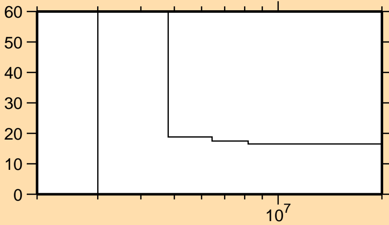
\Delta\sigma/\sigma vs. E for ^{62}\text{Ni}(n,p)
