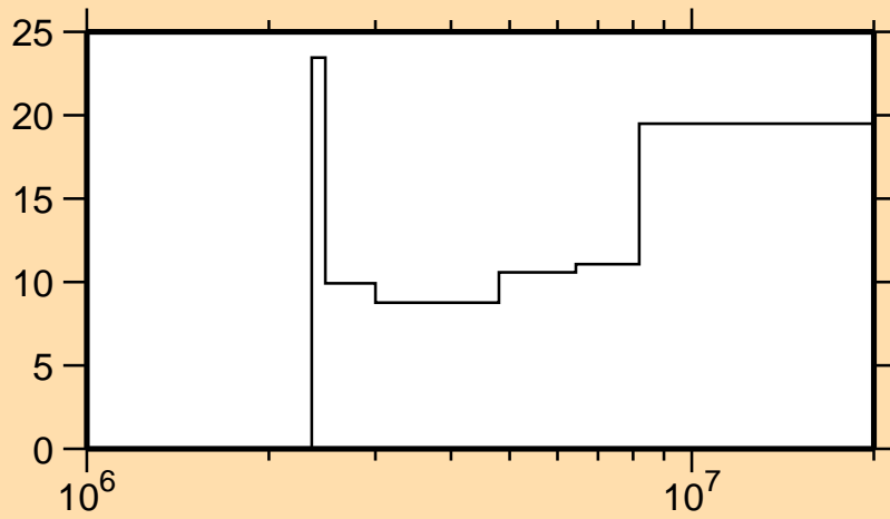
\Delta\sigma/\sigma vs. E for ^{62}\text{Ni}(n,n_4)
