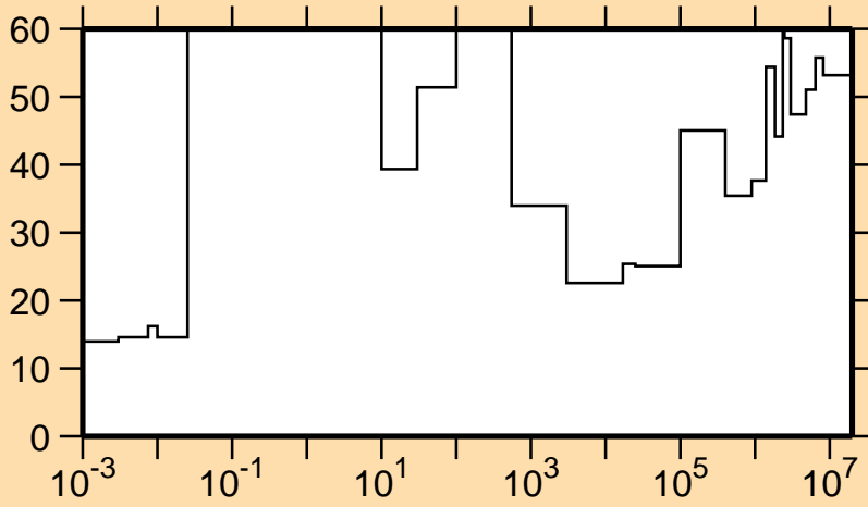
\Delta\sigma/\sigma vs. E for ^{62}\text{Ni}(n,\gamma)
