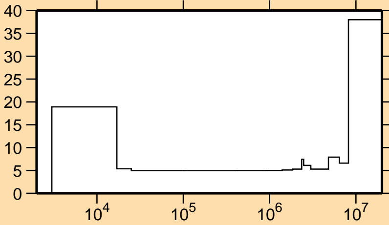
\Delta\sigma/\sigma vs. E for ^{57}\text{Fe}(n,n_1)
