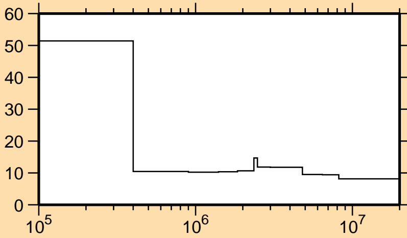
\Delta\sigma/\sigma vs. E for ^{57}\text{Fe}(n,n_3)
