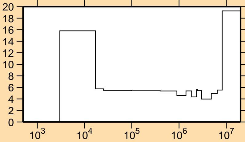
\Delta\sigma/\sigma vs. E for ^{57}\text{Fe}(n,\text{inel.})
