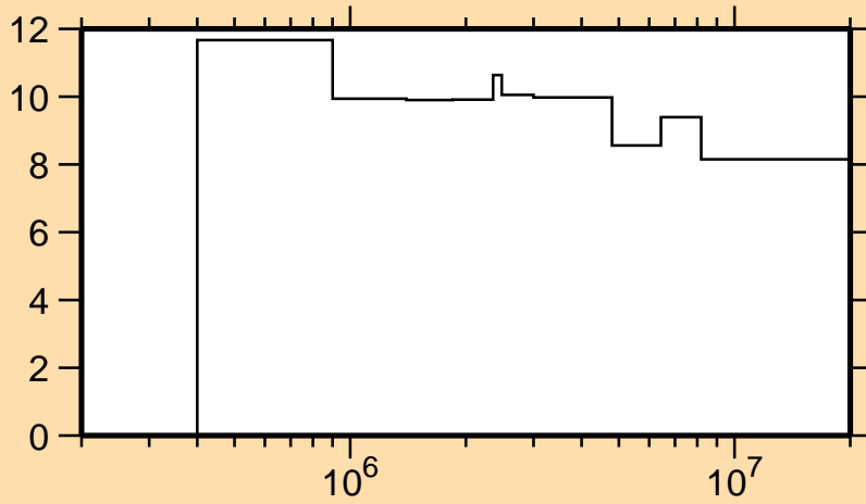
\Delta\sigma/\sigma vs. E for ^{57}\text{Fe}(n,n_4)
