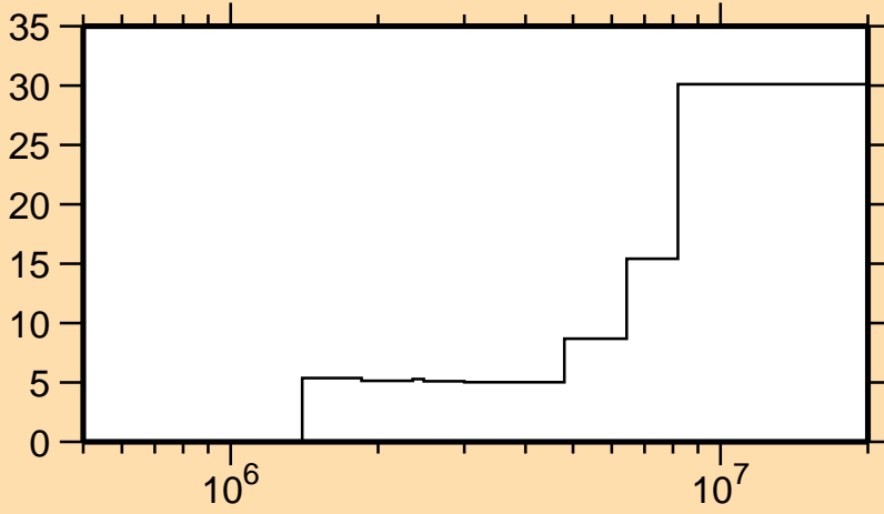
\Delta\sigma/\sigma vs. E for ^{54}\text{Fe}(n,n_1)
