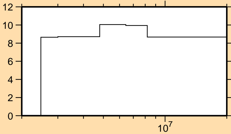
\Delta\sigma/\sigma vs. E for ^{54}\text{Fe}(n,n_3)
