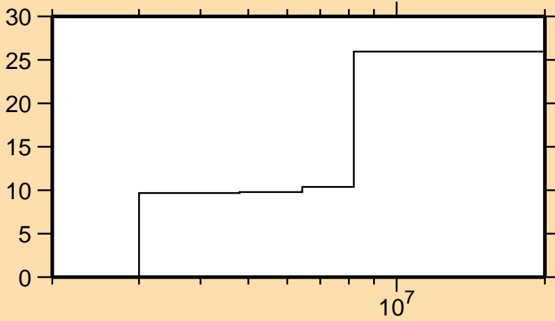
\Delta\sigma/\sigma vs. E for ^{54}\text{Fe}(n,n_7)
