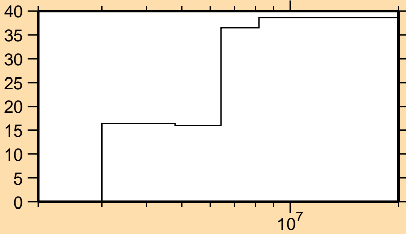
\Delta\sigma/\sigma vs. E for ^{50}\text{Ti}(n,n_3)
