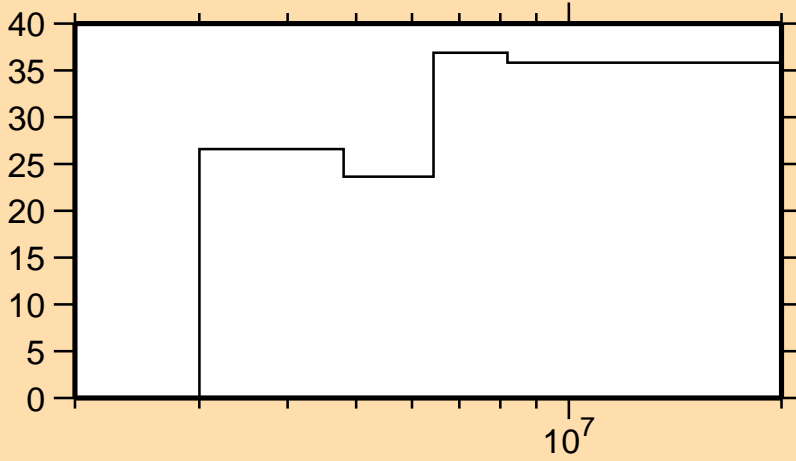
\Delta v/v vs. E for ^{50}\text{Ti}(\text{mt854})
