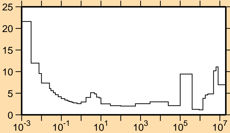
\Delta\sigma/\sigma vs. E for ^{50}\text{Ti}(n,\text{el.})
