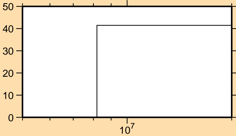
\Delta\sigma/\sigma vs. E for ^{50}\text{Ti}(n,np)
