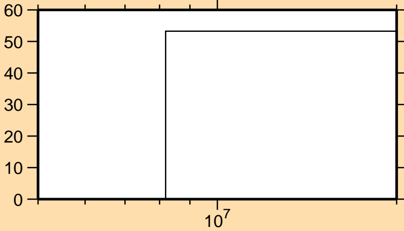
\Delta\sigma/\sigma vs. E for ^{50}\text{Ti}(n,d)
