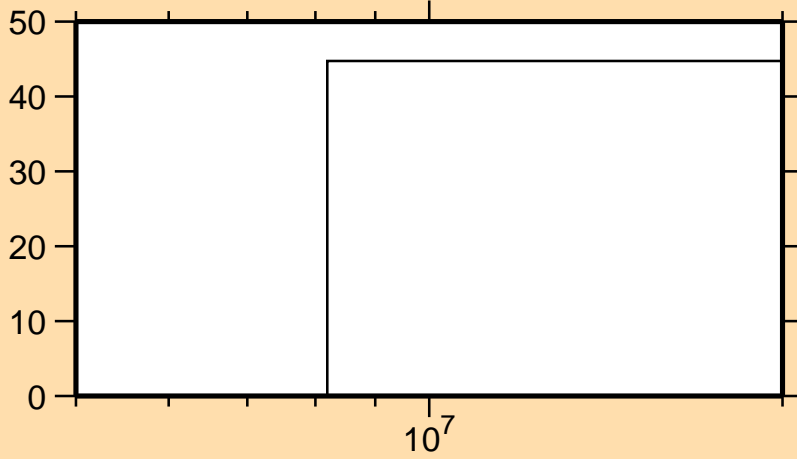
\Delta\sigma/\sigma vs. E for ^{50}\text{Ti}(n,n\alpha)
