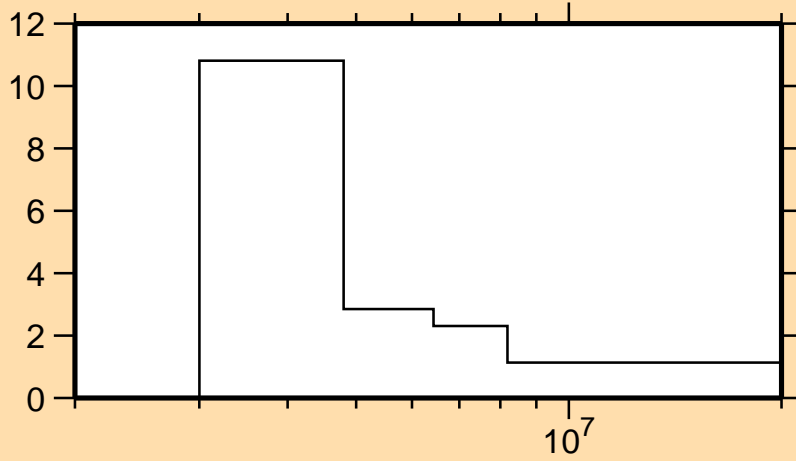
\Delta\sigma/\sigma vs. E for ^{48}\text{Ti}(n,p)
