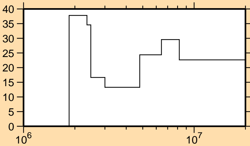
\Delta v/v vs. E for ^{48}\text{Ti}(\text{mt851})
