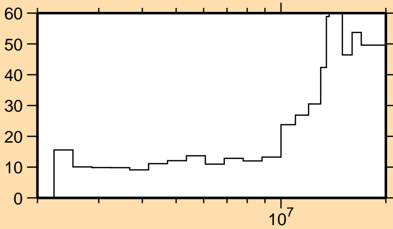
\Delta\sigma/\sigma vs. E for ^{62}\text{Ni}(n,n_4)
