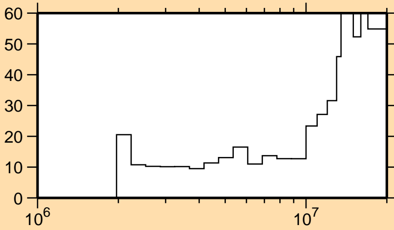
\Delta\sigma/\sigma vs. E for ^{62}\text{Ni}(n,n_2)
