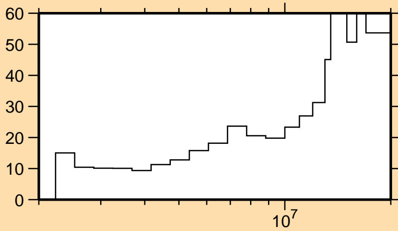
\Delta\sigma/\sigma vs. E for ^{62}\text{Ni}(n,n_3)
