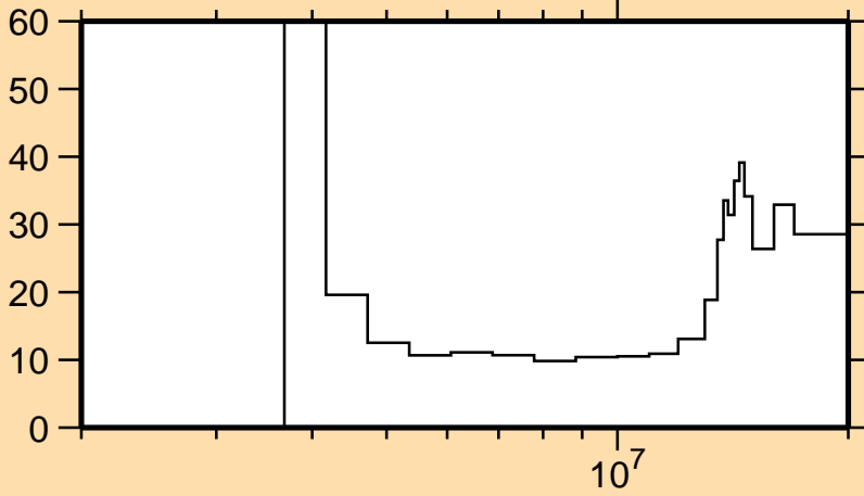
\Delta\sigma/\sigma vs. E for ^{58}\text{Fe}(n,n\text{cont.})
