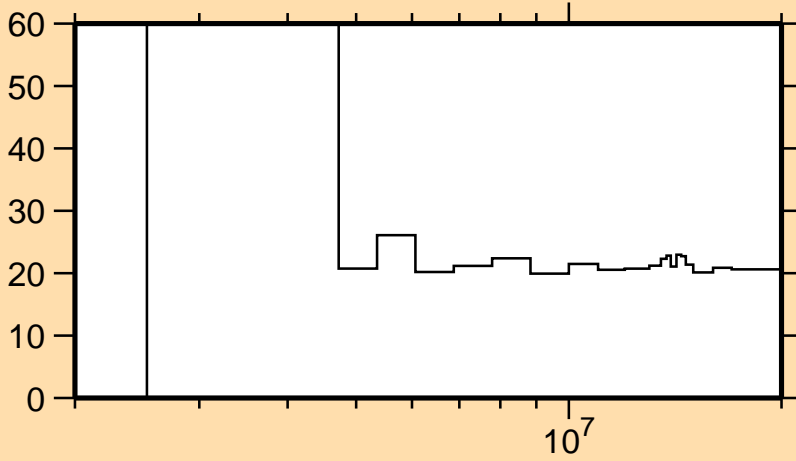
\Delta\sigma/\sigma vs. E for ^{58}\text{Fe}(n,\alpha)
