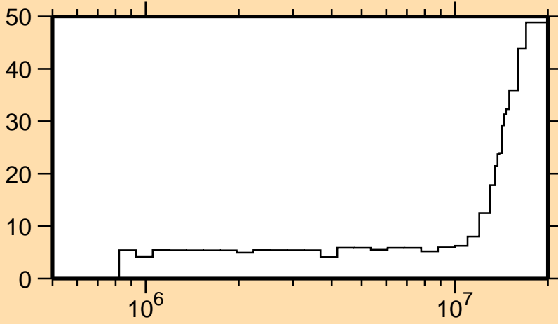
\Delta\sigma/\sigma vs. E for ^{58}\text{Fe}(n,\text{inel.})
