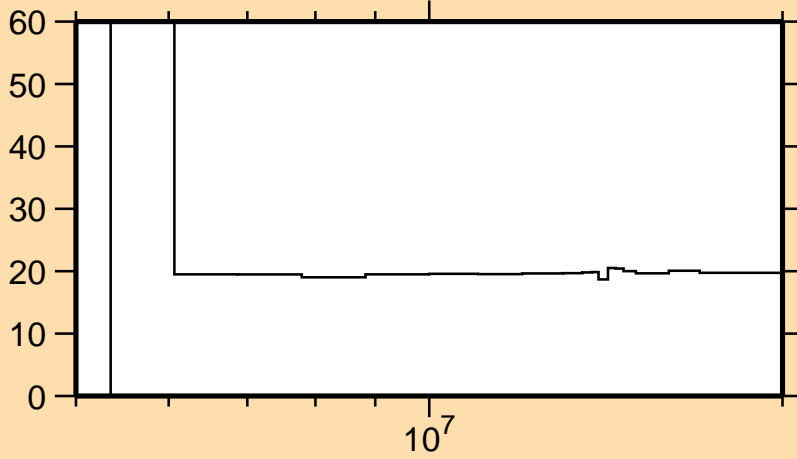
\Delta\sigma/\sigma vs. E for ^{58}\text{Fe}(n,p)
