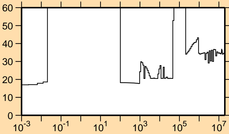
\Delta\sigma/\sigma vs. E for ^{57}\text{Fe}(n,\gamma)
