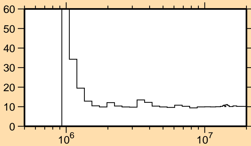
\Delta\sigma/\sigma vs. E for ^{57}\text{Fe}(n,\alpha)
