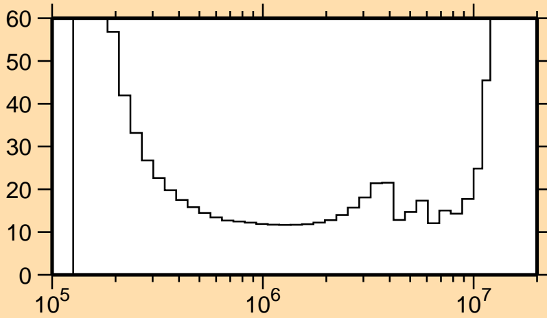
\Delta\sigma/\sigma vs. E for ^{57}\text{Fe}(n,n_2)
