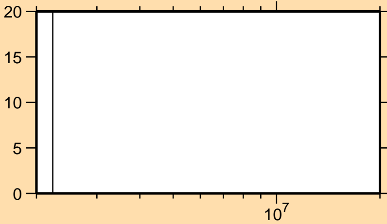
\Delta\sigma/\sigma vs. E for ^{55}\text{Mn}(n,n_{10})
