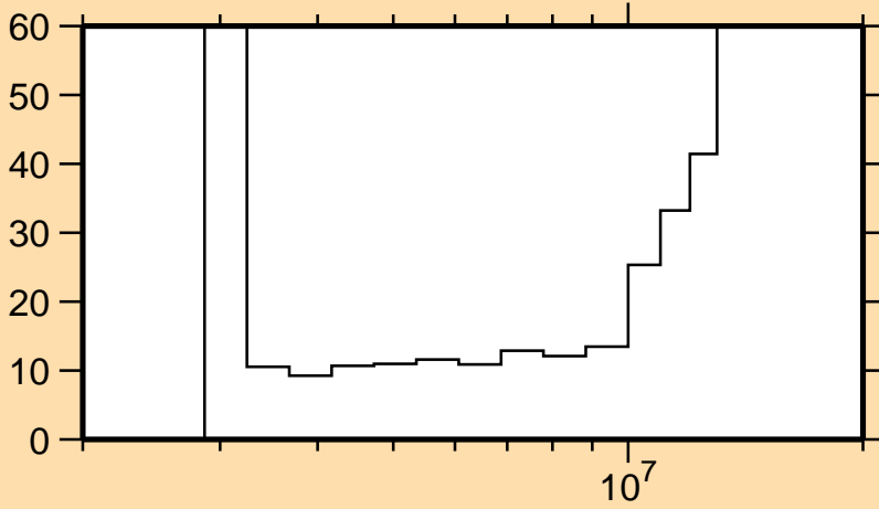
\Delta\sigma/\sigma vs. E for ^{50}\text{Cr}(n,n_4)
