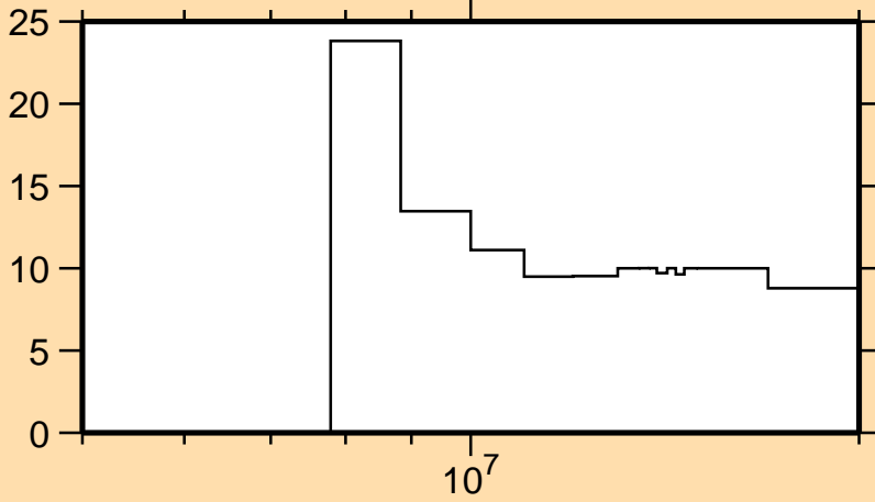
\Delta\sigma/\sigma vs. E for ^{49}\text{Ti}(n,2n)
