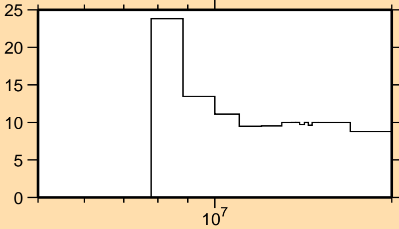
\Delta\sigma/\sigma vs. E for ^{49}\text{Ti}(n,2n)
