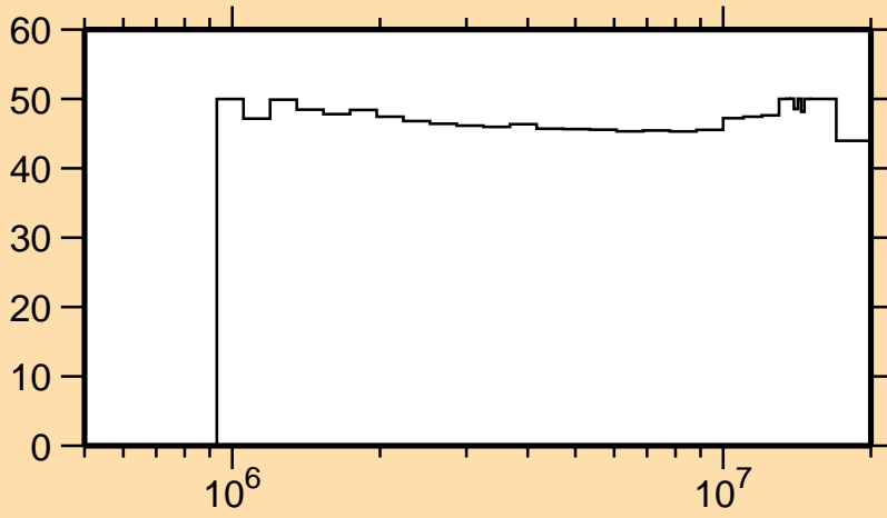
\Delta\sigma/\sigma vs. E for ^{49}\text{Ti}(n,\alpha)
