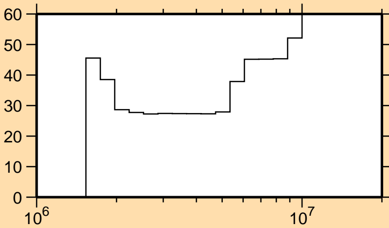
\Delta v/v vs. E for ^{49}\text{Ti}(\text{mt852})
