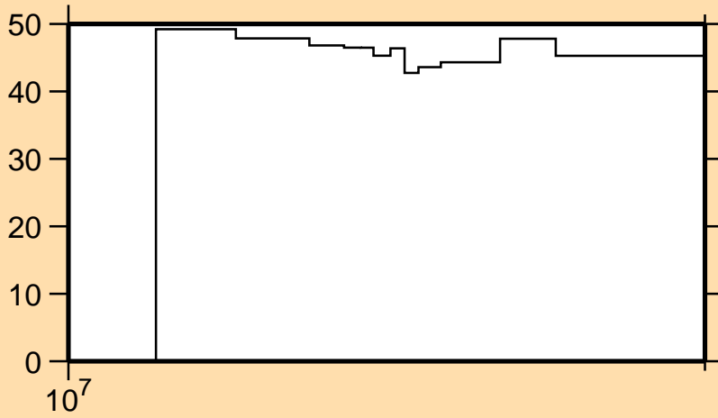
\Delta\sigma/\sigma vs. E for ^{49}\text{Ti}(n,np)
