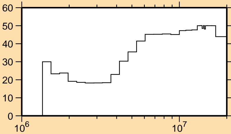
\Delta\sigma/\sigma vs. E for ^{49}\text{Ti}(n,n_1)
