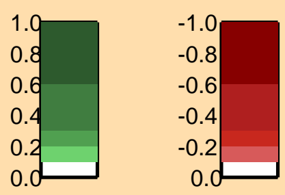
Correlation Matrix
