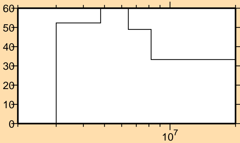
\Delta\sigma/\sigma vs. E for ^{156}\text{Gd}(n,p)
