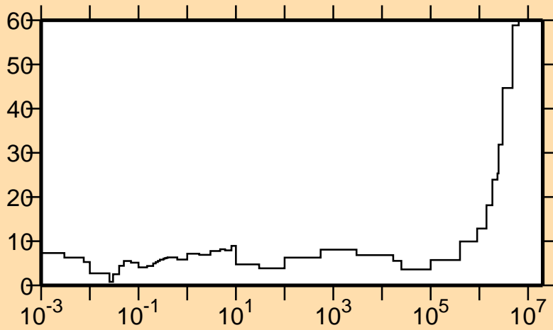
\Delta\sigma/\sigma vs. E for ^{155}\text{Gd}(n,\gamma)
