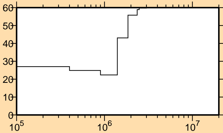
\Delta\sigma/\sigma vs. E for ^{154}\text{Gd}(n,\alpha)
