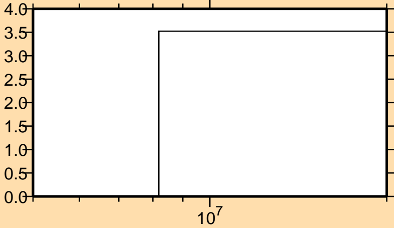
\Delta\sigma/\sigma vs. E for ^{89}\text{Y}(n,2n)
