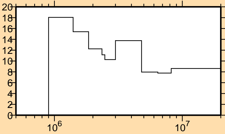
\Delta\sigma/\sigma vs. E for ^{89}\text{Y}(n,\text{inel.})
