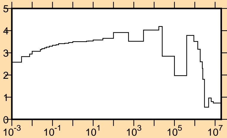
\Delta\sigma/\sigma vs. E for ^{89}\text{Y}(n,\text{tot.})
