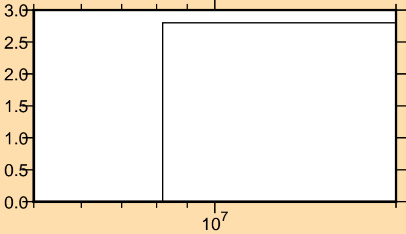
\Delta\sigma/\sigma vs. E for ^{58}\text{Ni}(n,2n)
