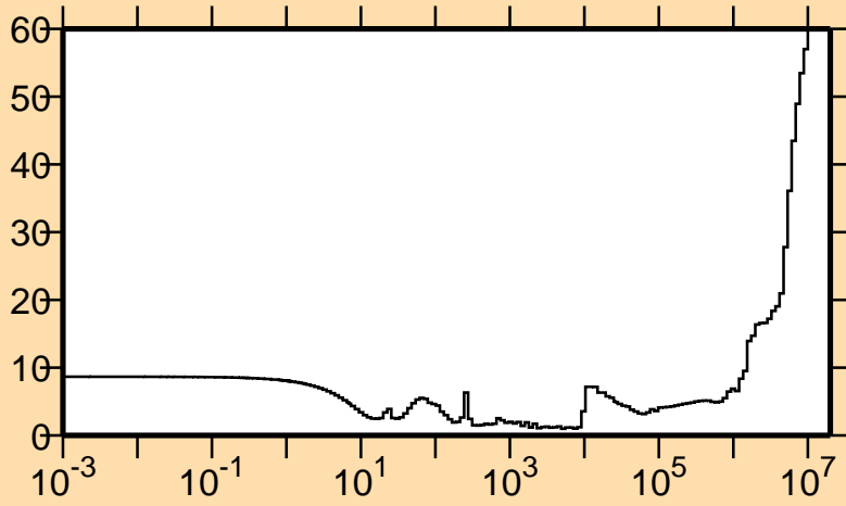
\Delta\sigma/\sigma vs. E for ^{158}\text{Gd}(n,\gamma)
