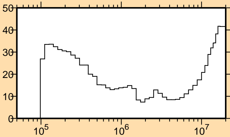
\Delta\sigma/\sigma vs. E for ^{156}\text{Gd}(n,\text{inel.})
