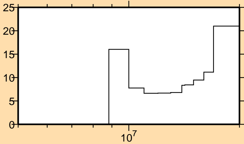
\Delta\sigma/\sigma vs. E for ^{156}\text{Gd}(n,2n)
