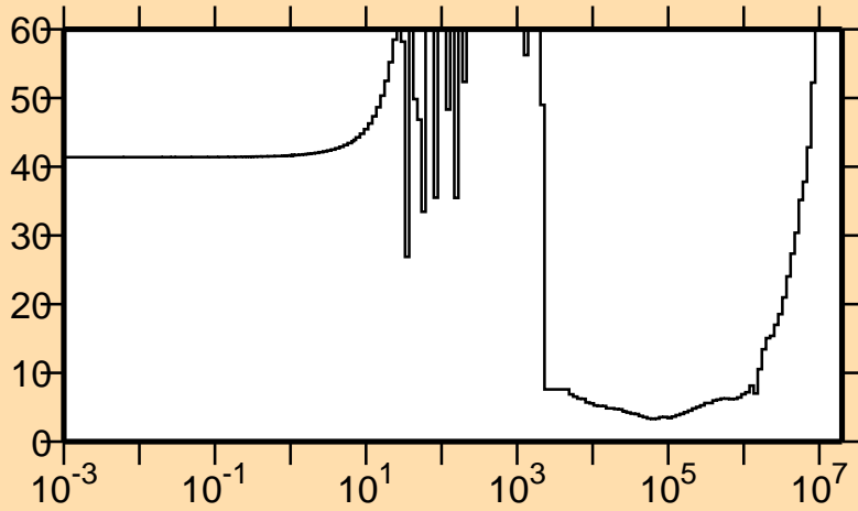
\Delta\sigma/\sigma vs. E for ^{156}\text{Gd}(n,\gamma)
