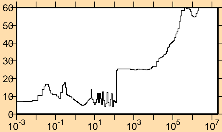
\Delta\sigma/\sigma vs. E for ^{153}\text{Gd}(n,\gamma)
