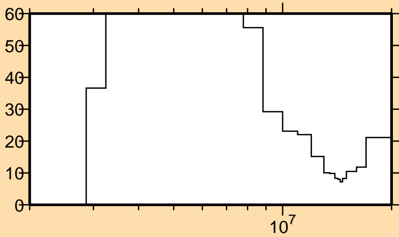
\Delta\sigma/\sigma vs. E for ^{89}\text{Y}(n,\alpha)
