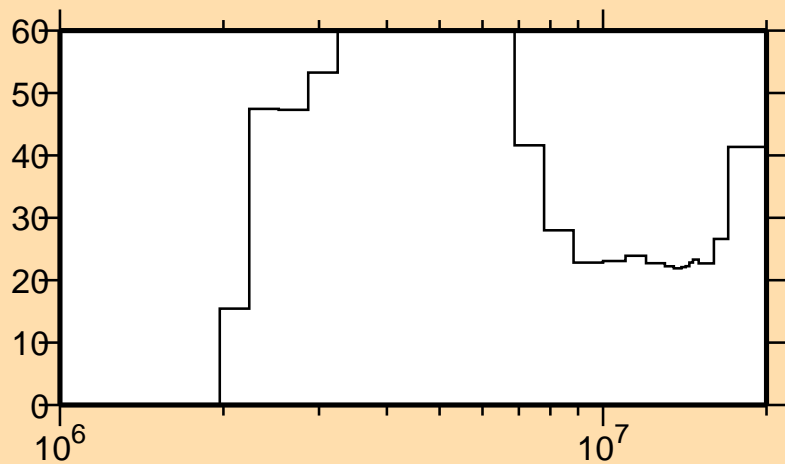
\Delta\sigma/\sigma vs. E for ^{89}\text{Y}(n,p)
