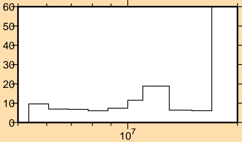
\Delta v/v vs. E for {}^7\text{Li}(\text{mt855})
