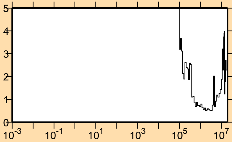
\Delta\sigma/\sigma vs. E for {}^7\text{Li}(n,\text{el.})
