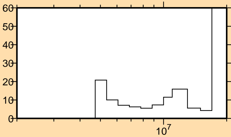
\Delta v/v vs. E for {}^7\text{Li}(\text{mt854})
