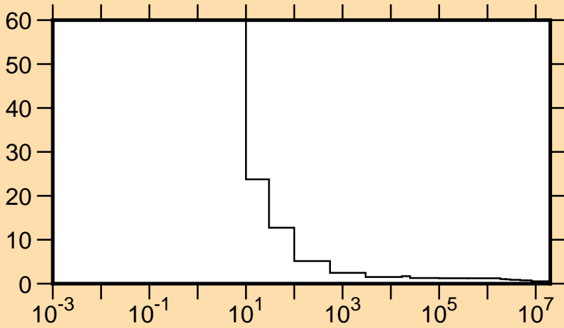
\Delta v/v vs. E for ^{240}\text{Pu} (total \nu )
