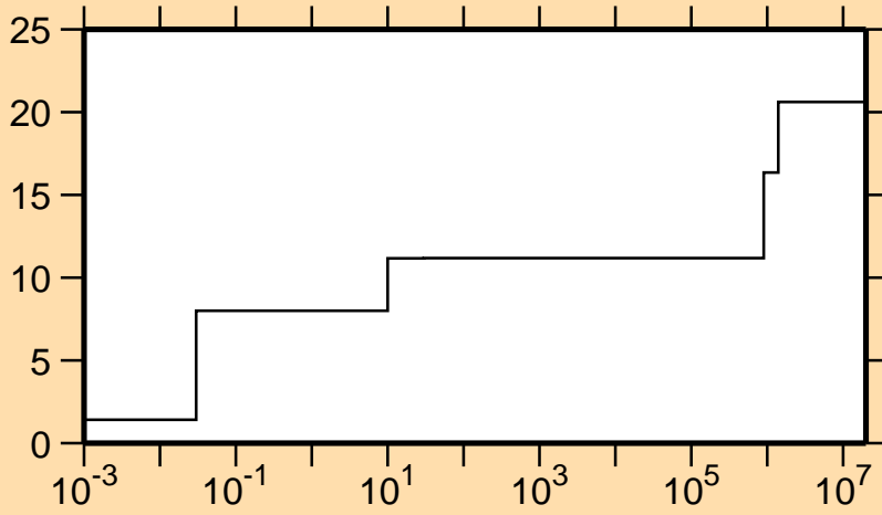
\Delta\sigma/\sigma vs. E for ^{232}\text{Th}(n,\gamma)
