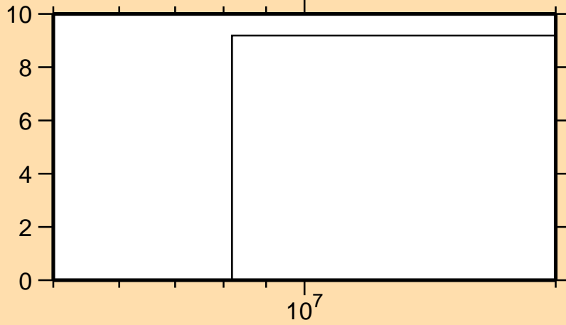
\Delta\sigma/\sigma vs. E for ^{93}\text{Nb}(n,3n)
