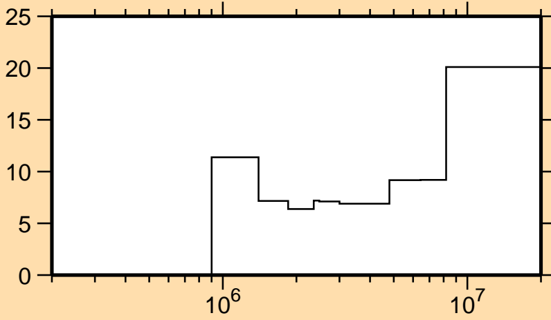
\Delta\sigma/\sigma vs. E for ^{64}\text{Ni}(n,\text{inel.})
