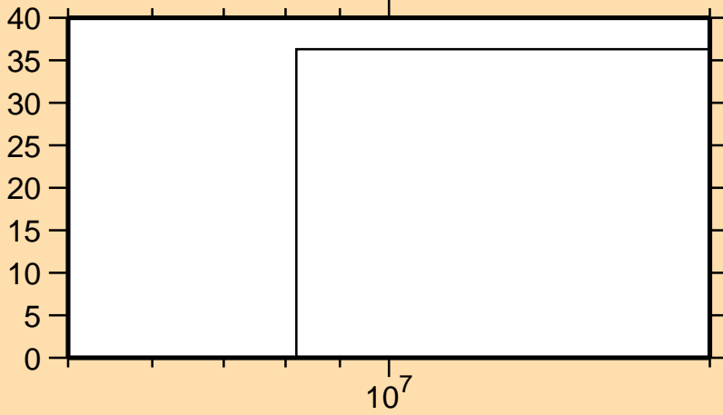
\Delta\sigma/\sigma vs. E for ^{64}\text{Ni}(n,np)
