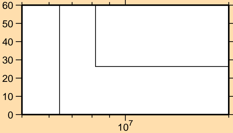
\Delta\sigma/\sigma vs. E for ^{64}\text{Ni}(n,p)
