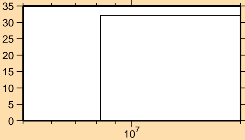
\Delta\sigma/\sigma vs. E for ^{64}\text{Ni}(n,d)
