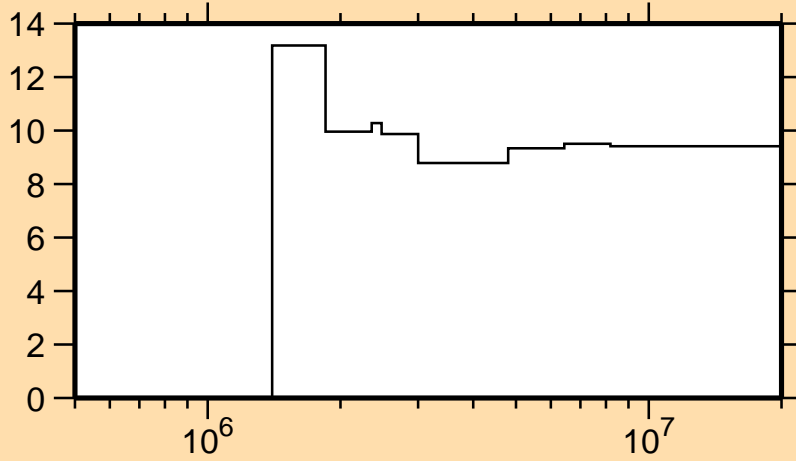
\Delta\sigma/\sigma vs. E for ^{58}\text{Fe}(n,n_2)
