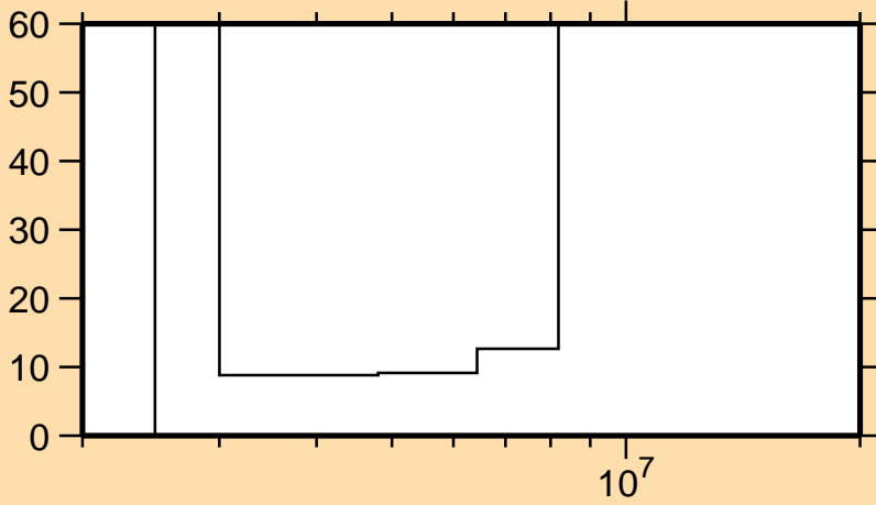
\Delta\sigma/\sigma vs. E for ^{56}\text{Fe}(n,n_4)
