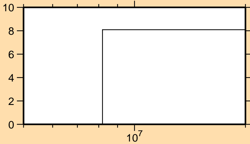
\Delta\sigma/\sigma vs. E for ^{56}\text{Fe}(n,2n)
