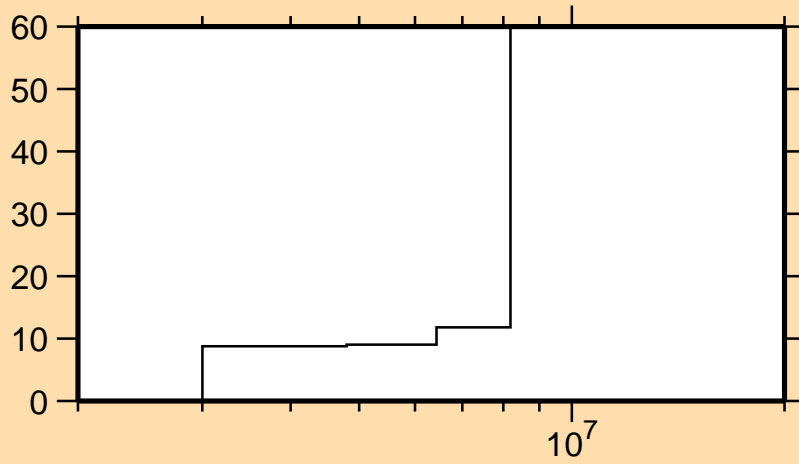
\Delta\sigma/\sigma vs. E for ^{56}\text{Fe}(n,n_5)
