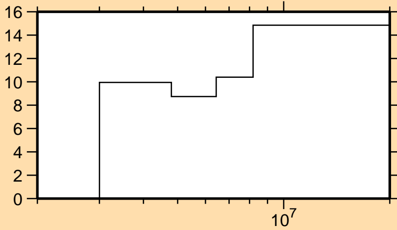
\Delta\sigma/\sigma vs. E for ^{56}\text{Fe}(n,n_{17})
