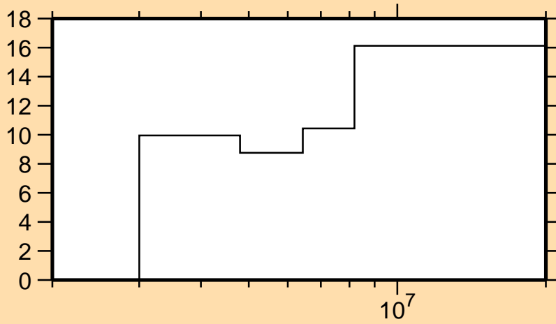
\Delta\sigma/\sigma vs. E for ^{56}\text{Fe}(n,n_{18})
