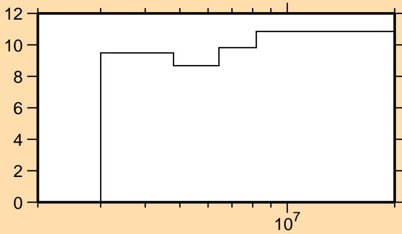
\Delta\sigma/\sigma vs. E for ^{56}\text{Fe}(n,n_g)
