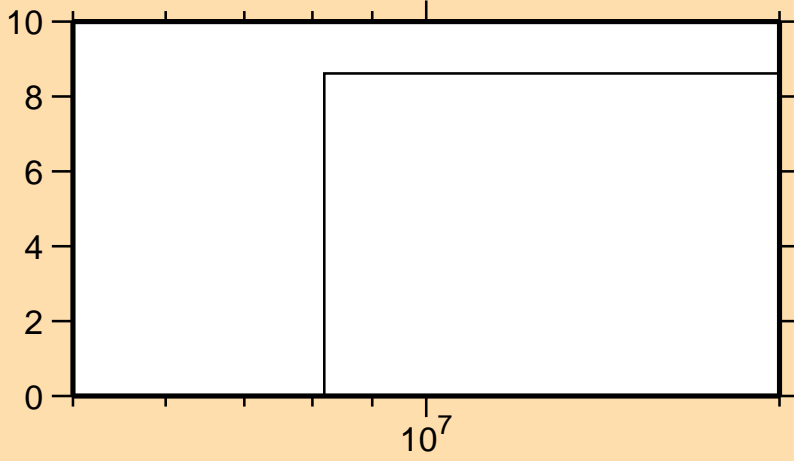
\Delta\sigma/\sigma vs. E for ^{54}\text{Fe}(n,2n)
