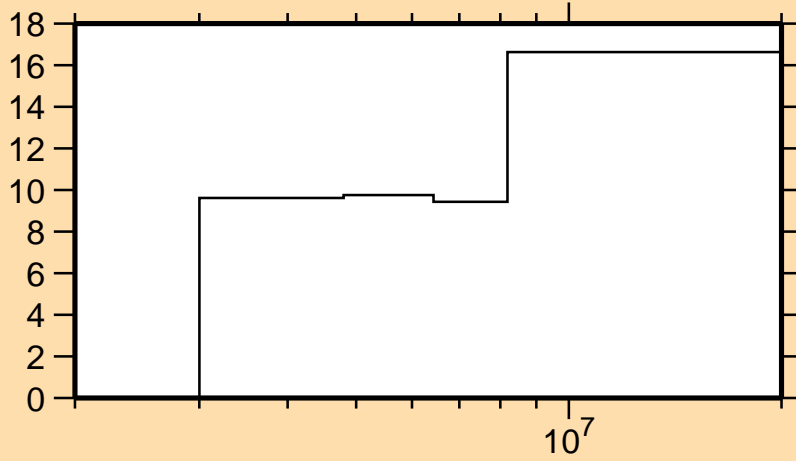
\Delta\sigma/\sigma vs. E for ^{54}\text{Fe}(n,n_4)
