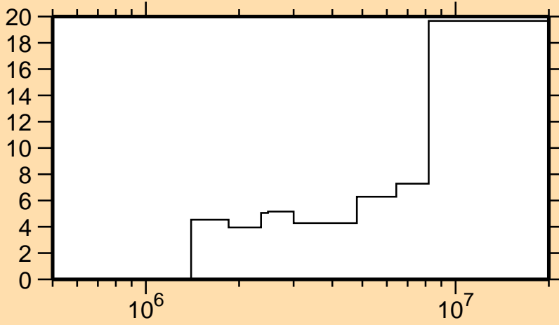
\Delta\sigma/\sigma vs. E for ^{54}\text{Fe}(n,\text{inel.})
