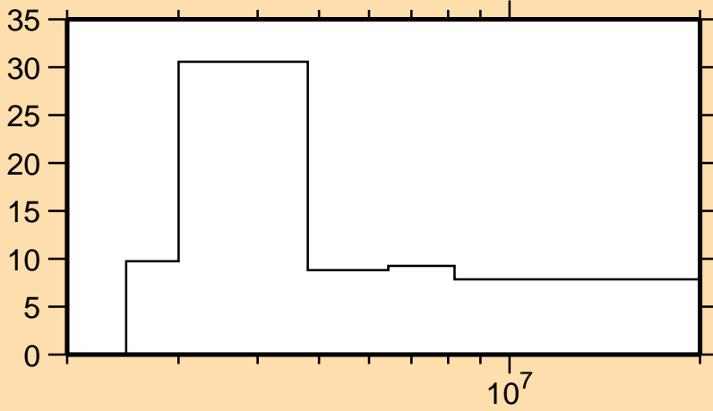
\Delta\sigma/\sigma vs. E for ^{54}\text{Fe}(n,\alpha)
