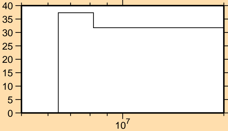
\Delta\sigma/\sigma vs. E for ^{54}\text{Fe}(n,d)
