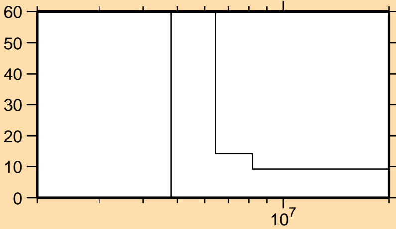
\Delta\sigma/\sigma vs. E for ^{54}\text{Cr}(n,p)
