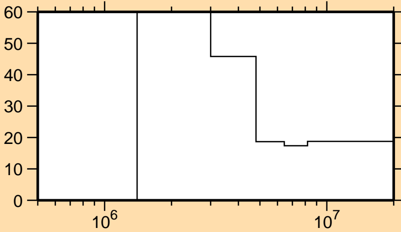
\Delta\sigma/\sigma vs. E for ^{54}\text{Cr}(n,\alpha)
