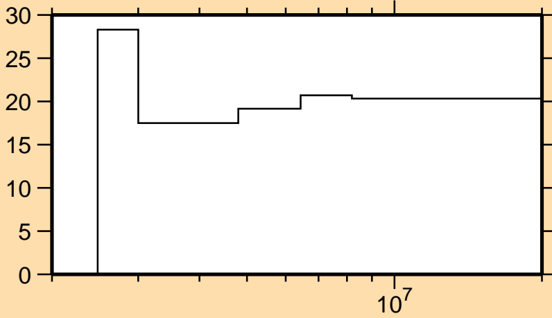
\Delta\sigma/\sigma vs. E for ^{53}\text{Cr}(n,n_{12})
