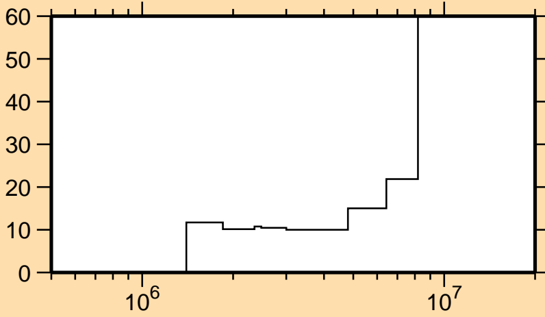
\Delta\sigma/\sigma vs. E for ^{53}\text{Cr}(n,n_4)
