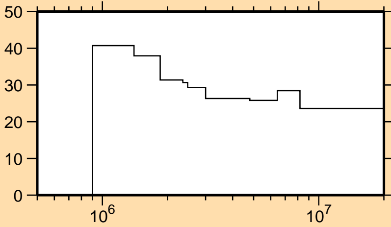
\Delta\sigma/\sigma vs. E for ^{53}\text{Cr}(n,\alpha)
