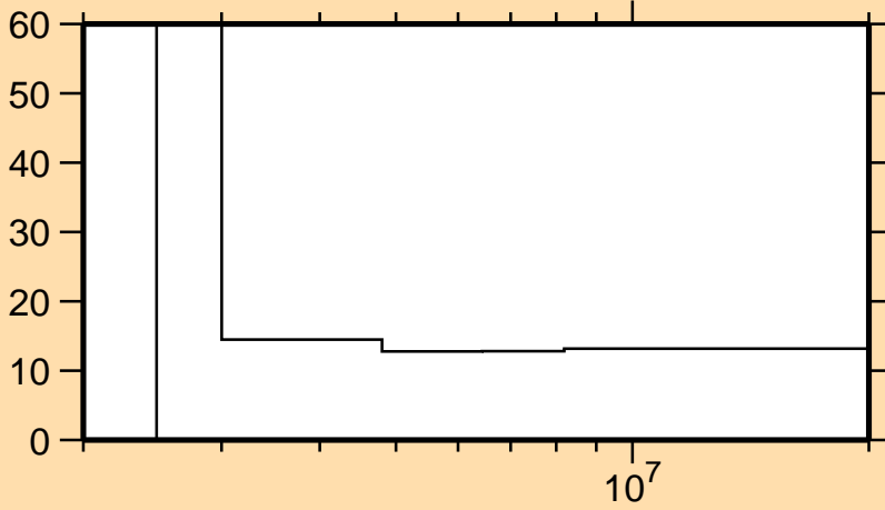
\Delta\sigma/\sigma vs. E for ^{53}\text{Cr}(n,p)
