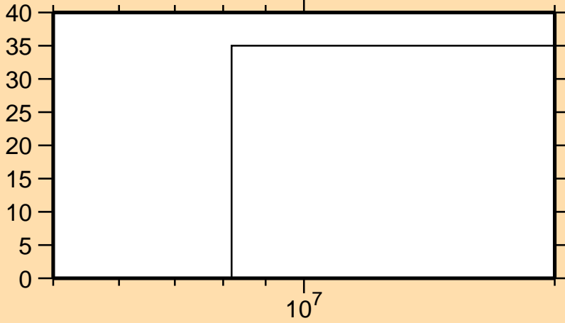
\Delta\sigma/\sigma vs. E for ^{19}\text{F}(n,t)
