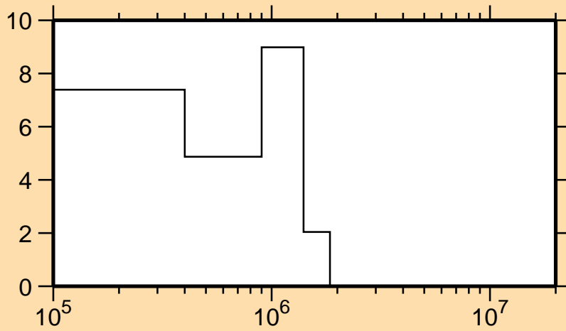
\Delta\sigma/\sigma vs. E for ^{19}\text{F}(n,n_1)
