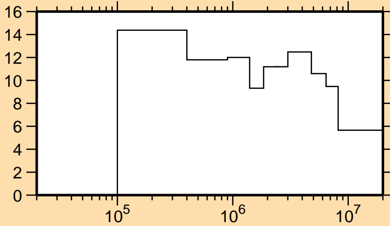
\Delta\sigma/\sigma vs. E for ^{19}\text{F}(n,\text{inel.})
