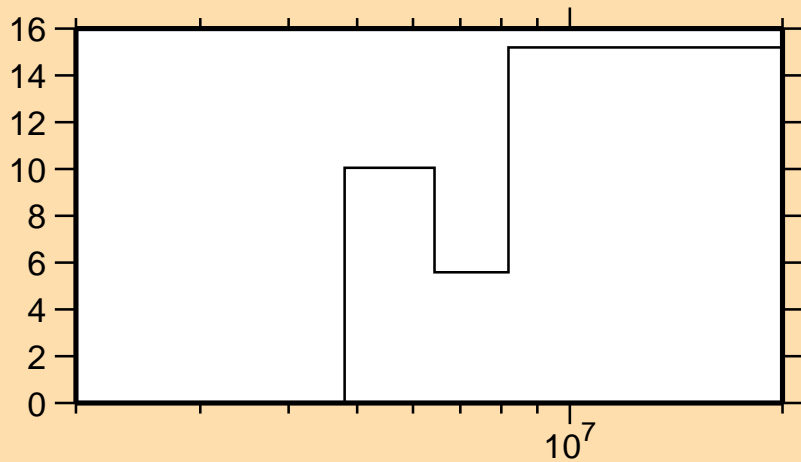
\Delta v/v vs. E for {}^7\text{Li}(\text{mt854})
