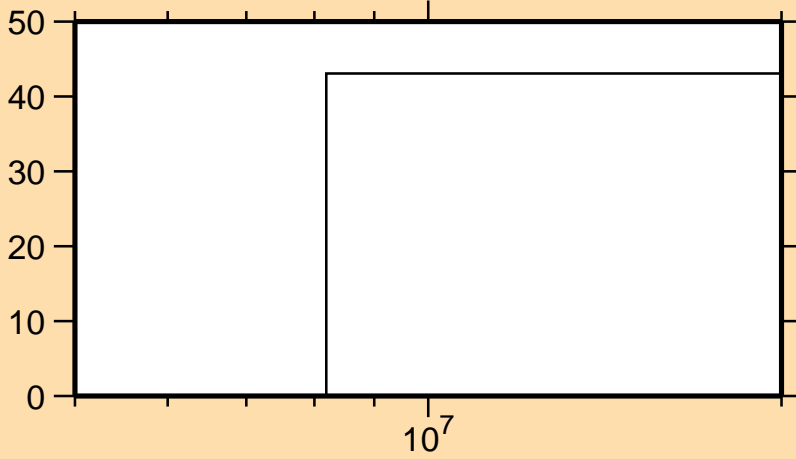
\Delta\sigma/\sigma vs. E for {}^7\text{Li}(n,3n\alpha)
