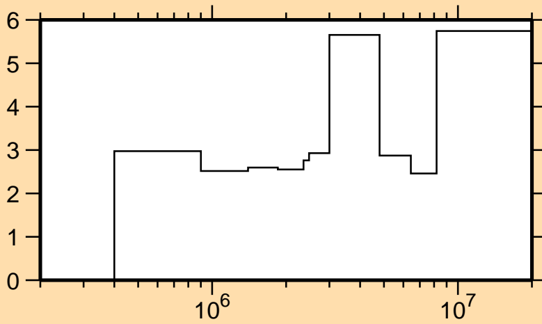
\Delta v/v vs. E for {}^7\text{Li}(\text{mt852})
