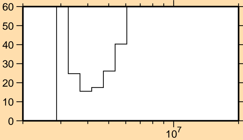
\Delta\sigma/\sigma vs. E for ^{208}\text{Pb}(n,n_2)
