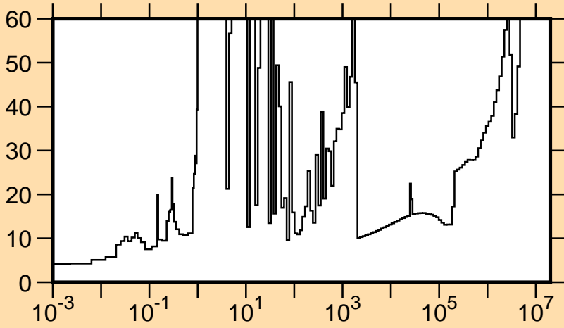
\Delta\sigma/\sigma vs. E for ^{187}\text{Re}(n,\gamma)
