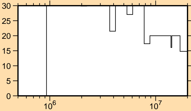
\Delta\sigma/\sigma vs. E for ^{89}\text{Y}(n,p)
