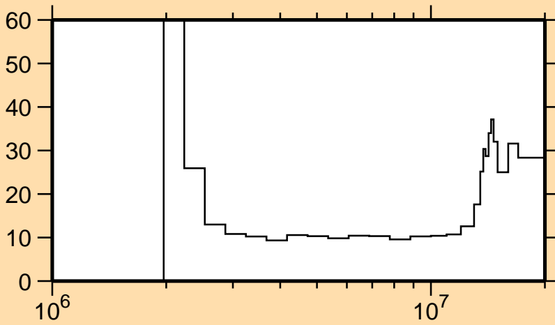
\Delta\sigma/\sigma vs. E for ^{58}\text{Fe}(n,n\text{cont.})
