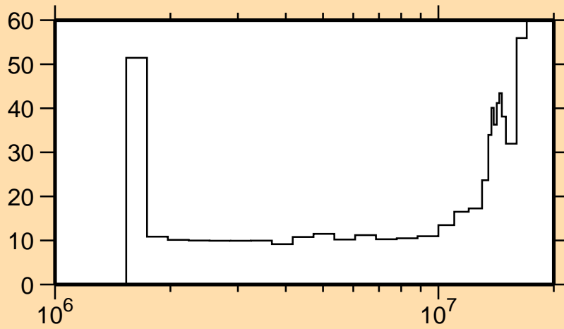
\Delta\sigma/\sigma vs. E for ^{58}\text{Fe}(n,n_2)
