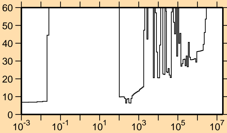
\Delta\sigma/\sigma vs. E for ^{58}\text{Fe}(n,\gamma)
