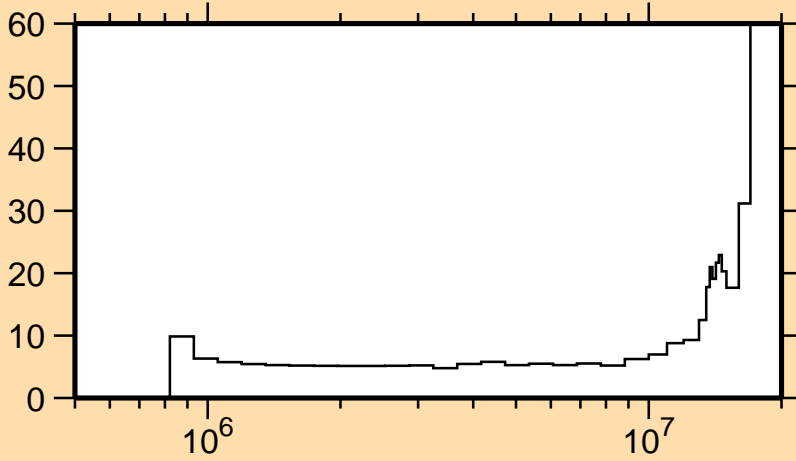
\Delta\sigma/\sigma vs. E for ^{58}\text{Fe}(n,n_1)
