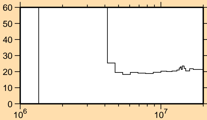
\Delta\sigma/\sigma vs. E for ^{58}\text{Fe}(n,\alpha)
