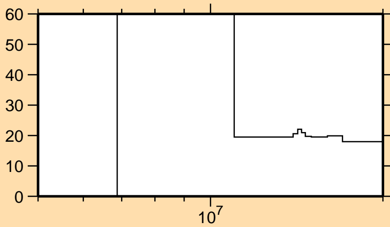
\Delta\sigma/\sigma vs. E for ^{58}\text{Fe}(n,n\alpha)
