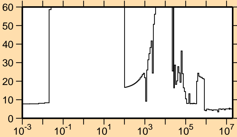
\Delta\sigma/\sigma vs. E for ^{56}\text{Fe}(n,\text{nonel.})
