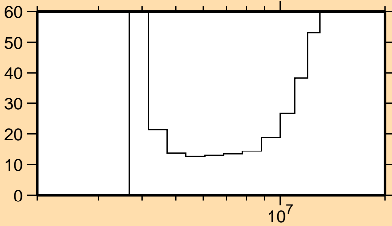
\Delta\sigma/\sigma vs. E for ^{56}\text{Fe}(n,n_{14})
