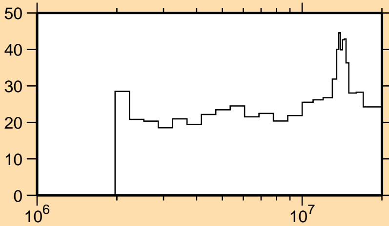
\Delta\sigma/\sigma vs. E for ^{53}\text{Cr}(n,n_5)
