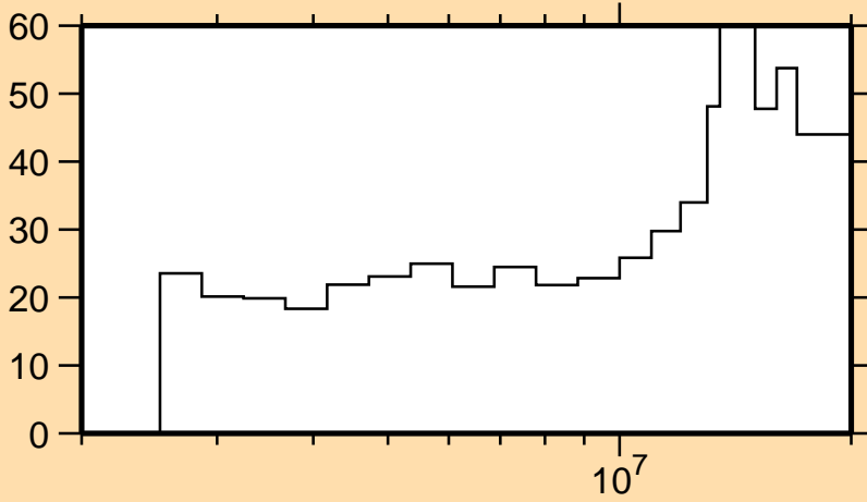
\Delta\sigma/\sigma vs. E for ^{53}\text{Cr}(n,n_{10})
