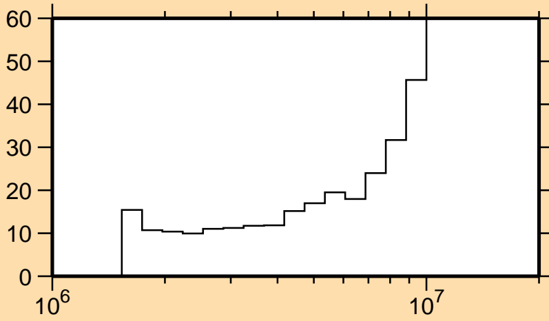
\Delta\sigma/\sigma vs. E for ^{53}\text{Cr}(n,n_4)
