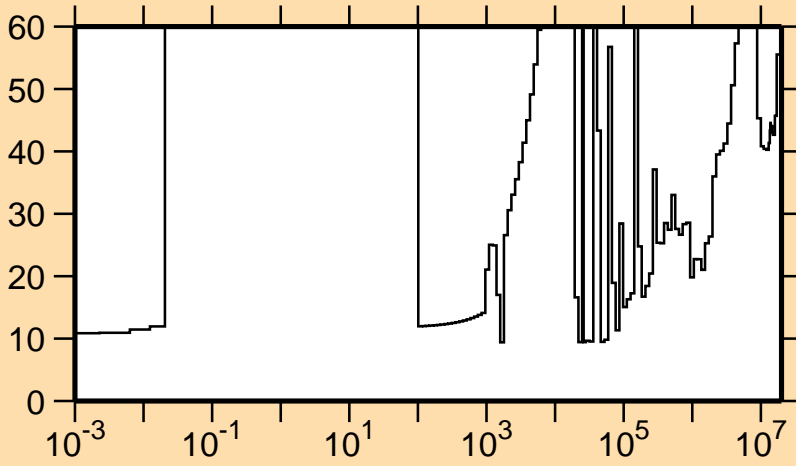
\Delta\sigma/\sigma vs. E for ^{52}\text{Cr}(n,\gamma)
