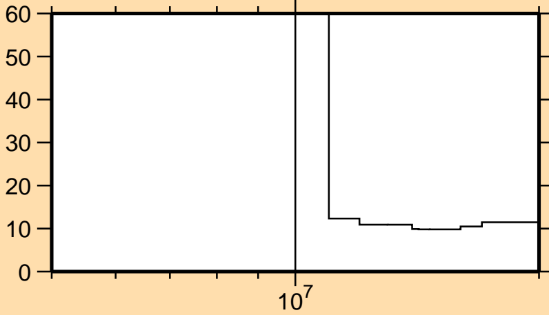
\Delta\sigma/\sigma vs. E for ^{19}\text{F}(n,2n)
