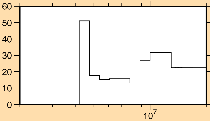
\Delta\sigma/\sigma vs. E for ^{19}\text{F}(n,p)
