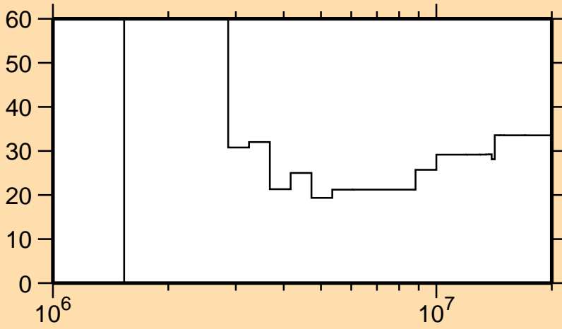
\Delta\sigma/\sigma vs. E for ^{19}\text{F}(n,\alpha)
