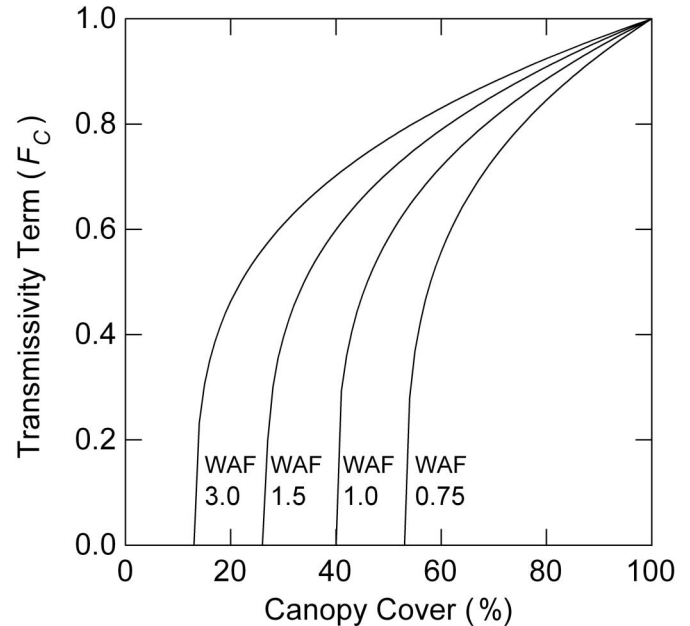
Fig. 2. Effect of canopy cover and wind speed adjustment factor (WAF) on crown-to-crown transmission of fire (eq. 10). Values of WAF > 1 decrease the threshold canopy cover (default, 40%) required for crown-to-crown transmission, and values of WAF < 1 increase the threshold canopy cover required for crown-to-crown transmission. At any single canopy cover, higher WAF values yield higher rates of crown-to-crown transmission. The greatest effect of wind speed occurs at low canopy covers.
