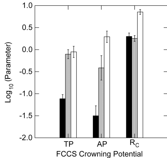
Fig. 10. Fuel Characteristic Classification System (FCCS) crown fire potentials (torching potential, TP, and active crowning potential, AP) and crown fire rate of spread, R_C , by fire type. The TP comparison is based on 86 FCCS conifer fuelbeds. The AP and R_C comparisons are based on 21 FCCS conifer fuelbeds in Alaska and the northeastern United States. Input parameters included estimated fine-fuel moisture content (EFFM) for TP comparisons ( N = 430 ) and wind speed for AP and R_C comparisons ( N = 252 ). Fire type was calculated from the Crown Fire Initiation and Spread (CFIS) model (Cruz et al. 2006b and 2006c; Alexander et al. 2006) using the FCCS fuelbed characteristics and environmental inputs, EFFM, and wind speed. Fire types consisted of surface (black bar), torching (gray bar), and active crown fire (open bar). Differences between fire types were statistically different for each of the potentials ( P < 0.001 ; zero values were set to a value of 10^{-2} or \log_{10} = -2 ). Error bars represent the 95% confidence interval.
