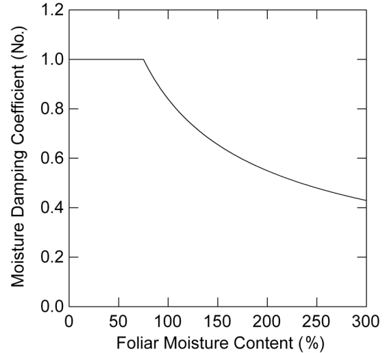
Fig. 5. Effect of canopy foliar moisture content (%) on the moisture damping coefficient and canopy flammability (eq. 25). The shape of this curve approximates the influence of foliar moisture content on canopy flammability in Van Wagner (1977).
