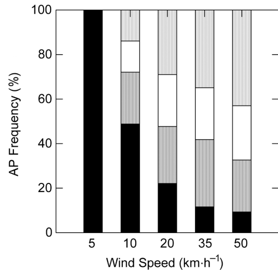
Fig. 8. Distribution of active crowning potential (AP) as a function of 10 m open wind speed based on 21 Fuel Characteristic Classification System (FCCS) conifer fuelbeds in Alaska and the north-eastern United States. Classes shown are 0 (black), 0–1 (dark gray), 1–6 (open), and 6–10 (light gray).
