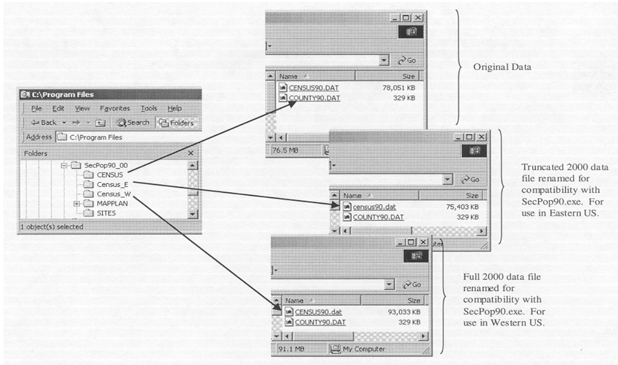
Figure 5-4 Verification Directory Structure
