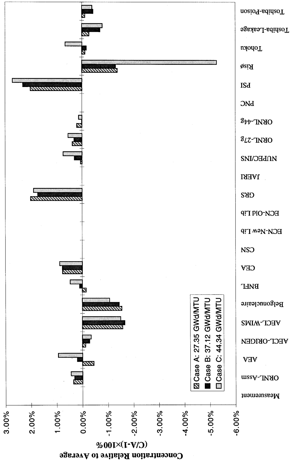
Fig. 15. Relative Ru-101 concentrations.
