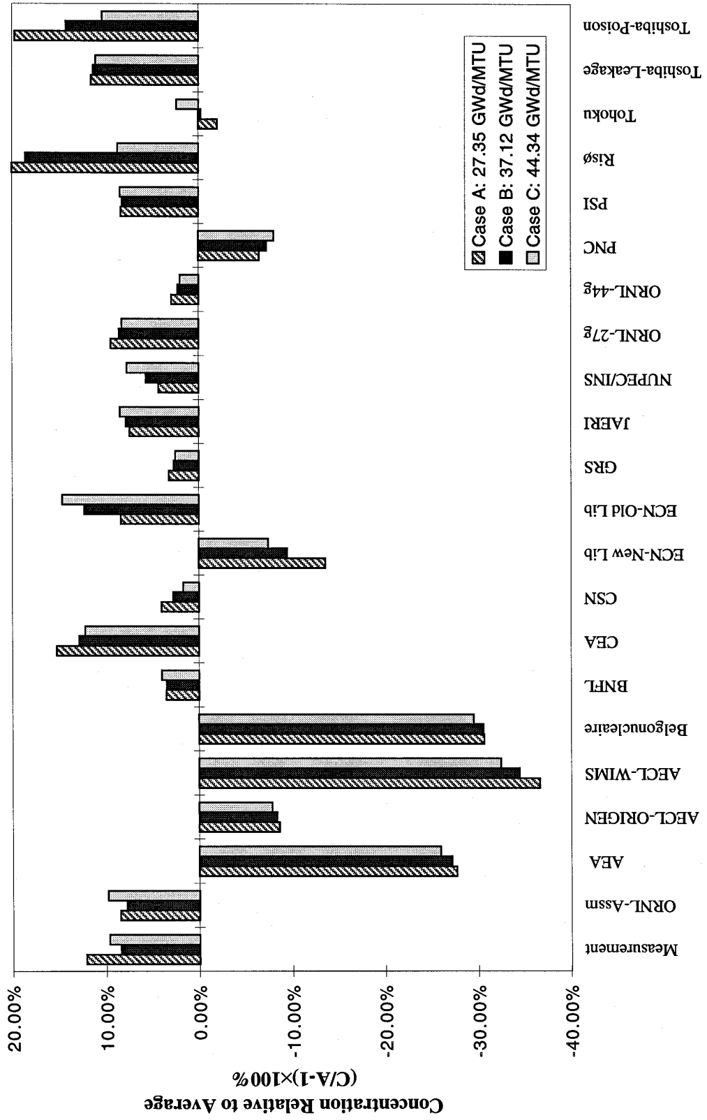
Fig. 5. Relative Pu-238 concentrations.
