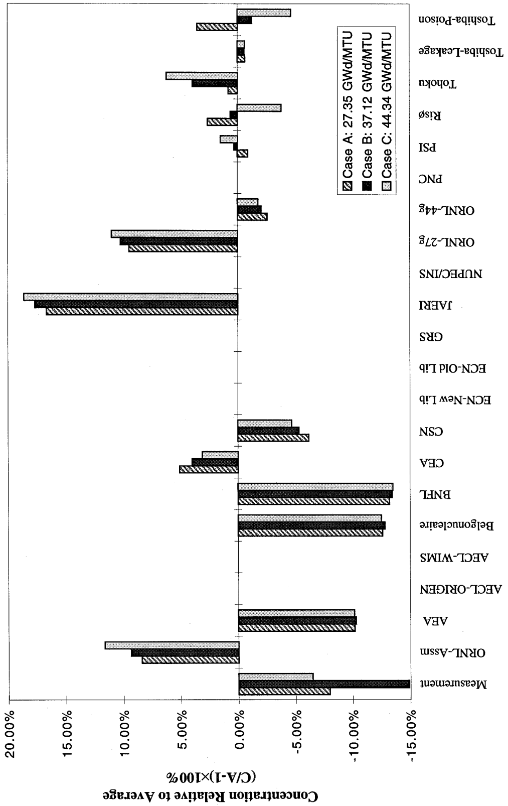
Fig. 12. Relative Np-237 concentrations.
