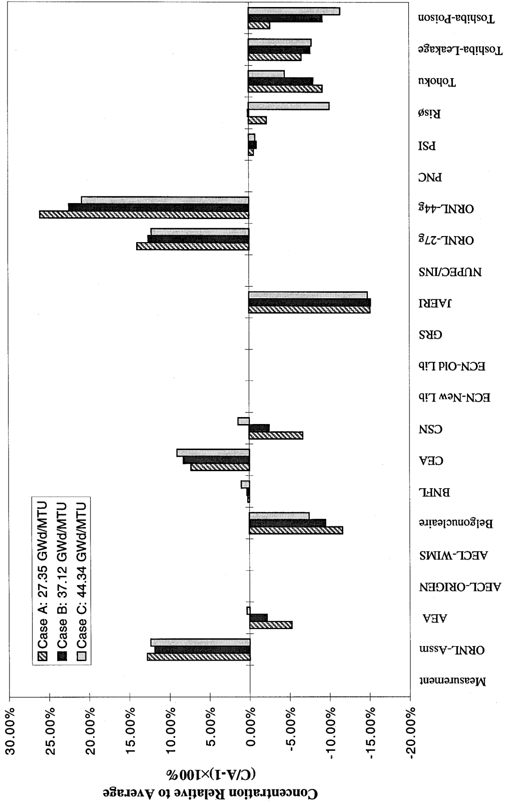
Fig. 11. Relative Am-243 concentrations.
