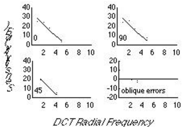
Figure 4. DCT basis function sensitivities at 64 pixels/degree.
