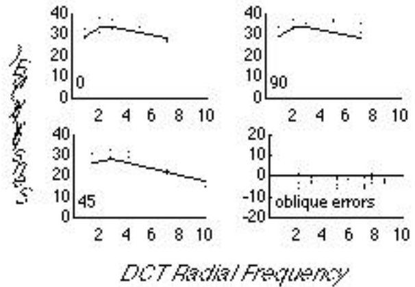
Figure 2. DCT basis function sensitivities at 16 pixels/degree.
