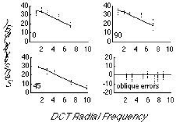
Figure 3. DCT basis function sensitivities at 32 pixels/degree.
