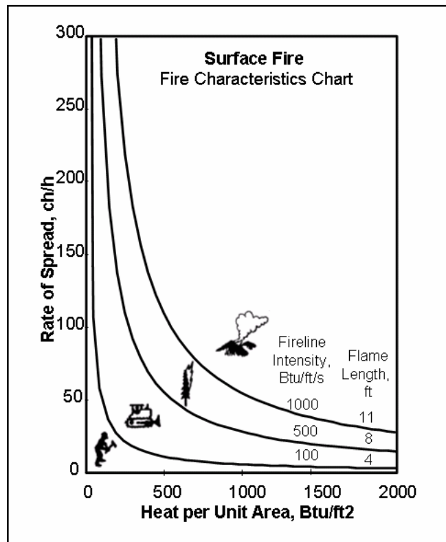
Figure 5—The fire characteristics chart shows the relationship among rate of spread, heat per unit area, fireline intensity, and flame length.
