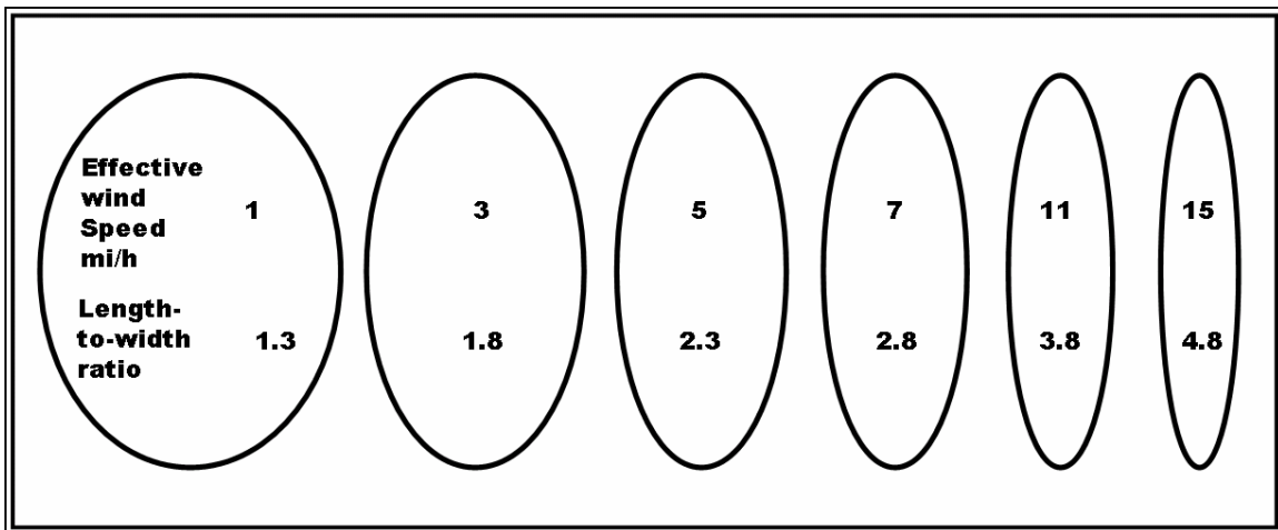
Figure 11—Fire shape depends on effective wind speed. Higher winds result in a higher length-to-width ratio.
