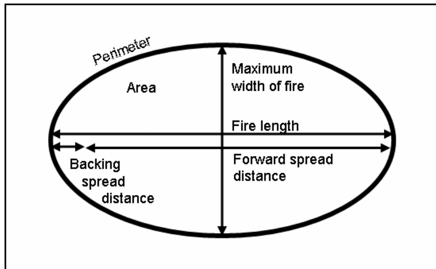
Figure 10—A point source fire shape and size is assumed to be elliptically shaped.
