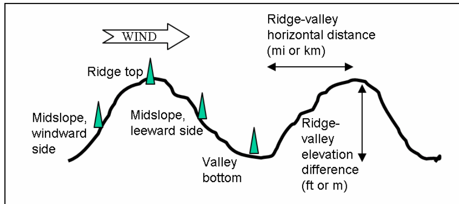
Figure 12—Terrain is described as a simplified sine shape for the spotting distance model.
