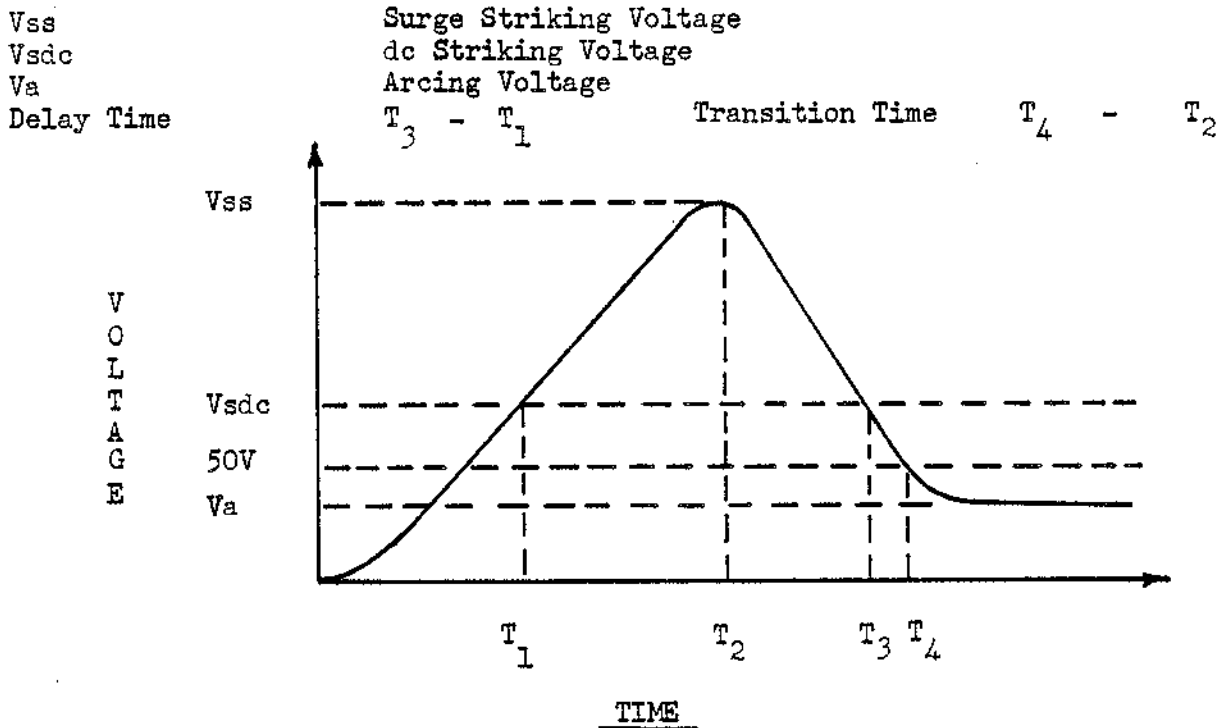
FIGURE 2: ARRESTER BREAKDOWN NOMENCLATURE
